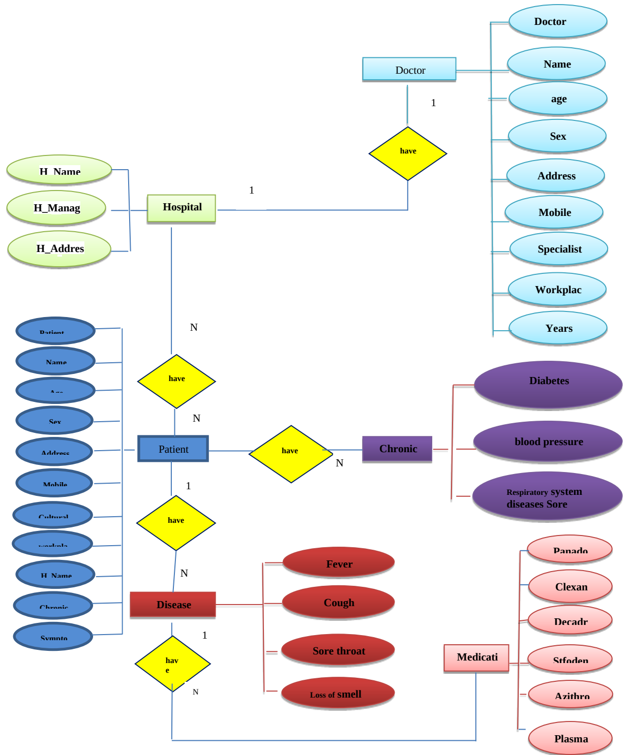
Figure 1: The ER-Diagram
