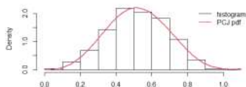
Fig 2: Estimated PDF and histogram for generated samples using the scenario (9, 3.5).
